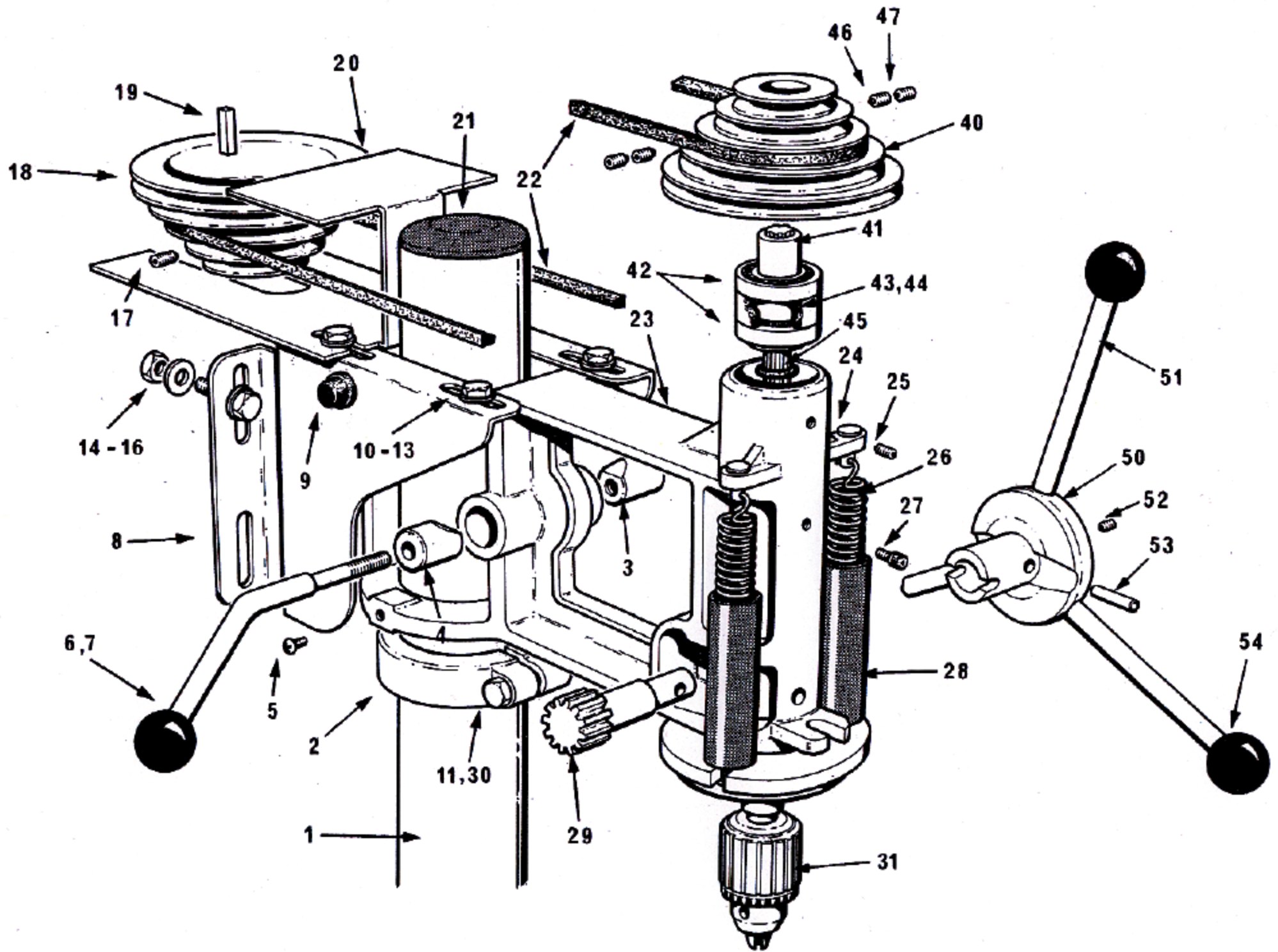
General Assembly
