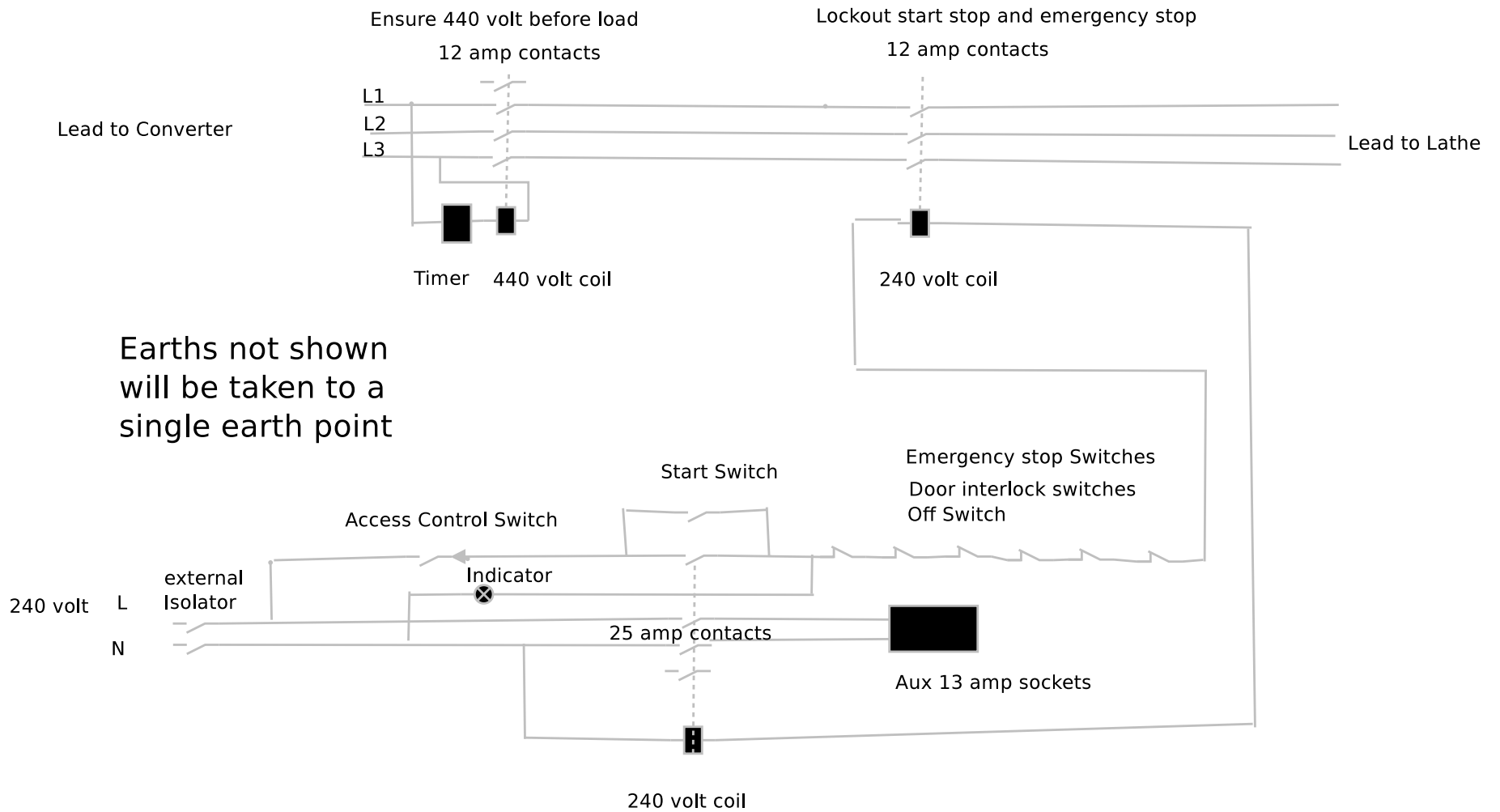
Hardinge Lathe Switch diagram - J Willis V2 2016-12-10
